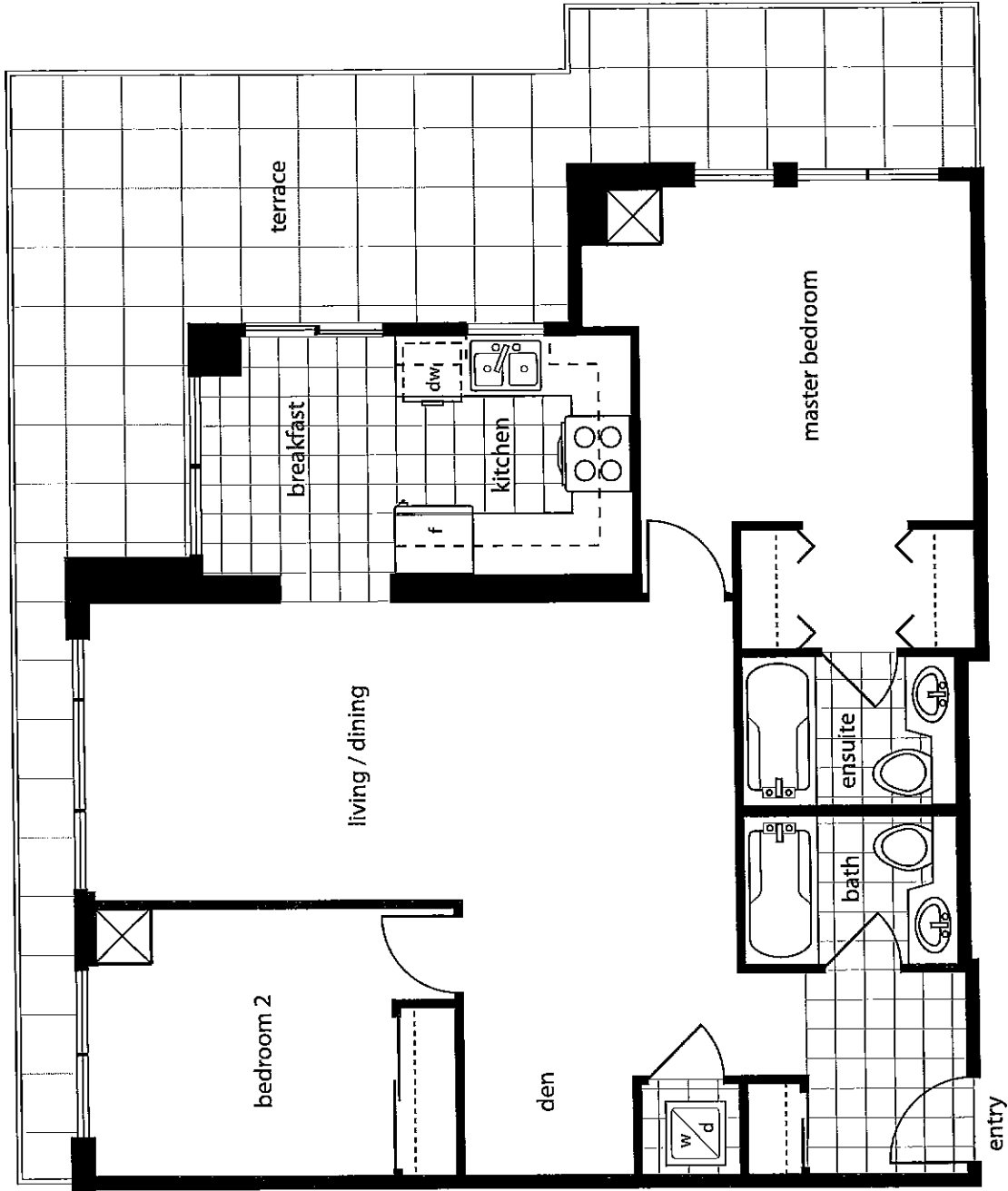
floorplan five (terrace):
