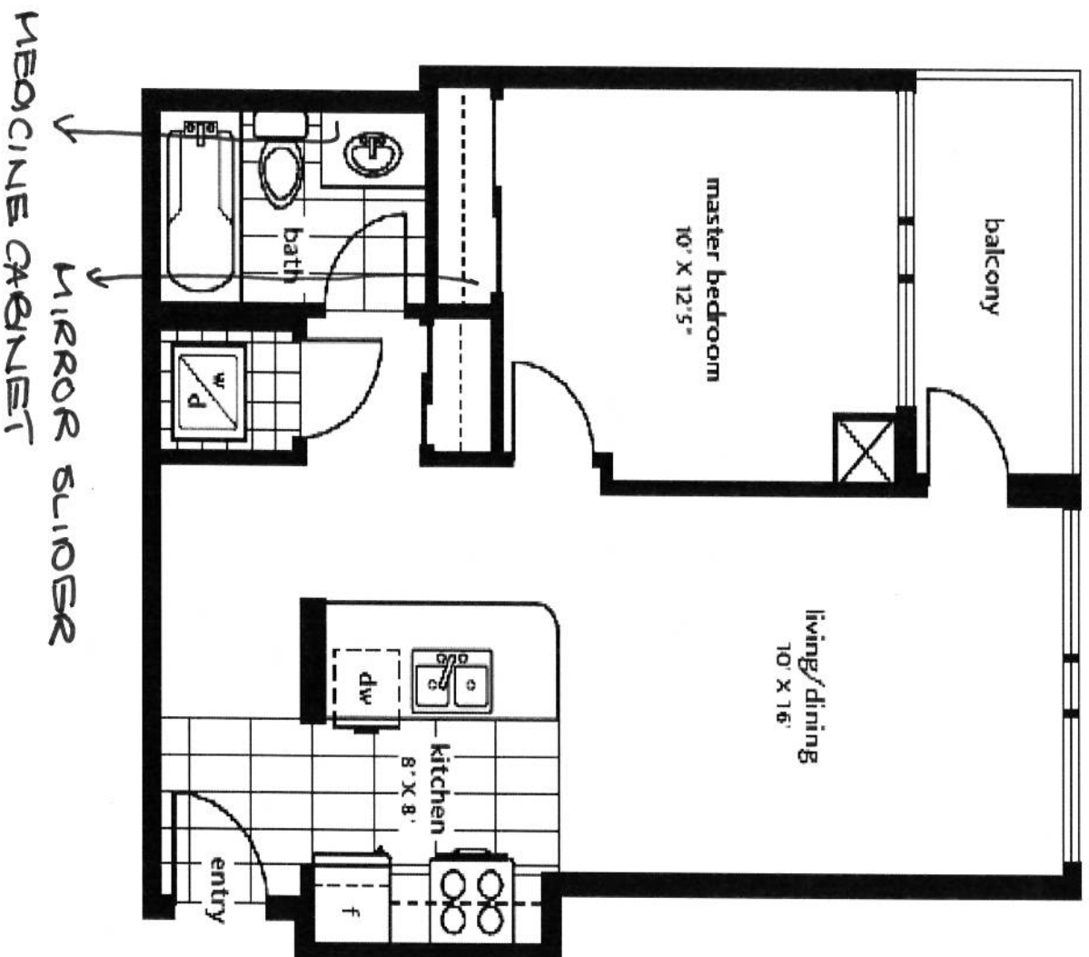
Floor Plan: 1
