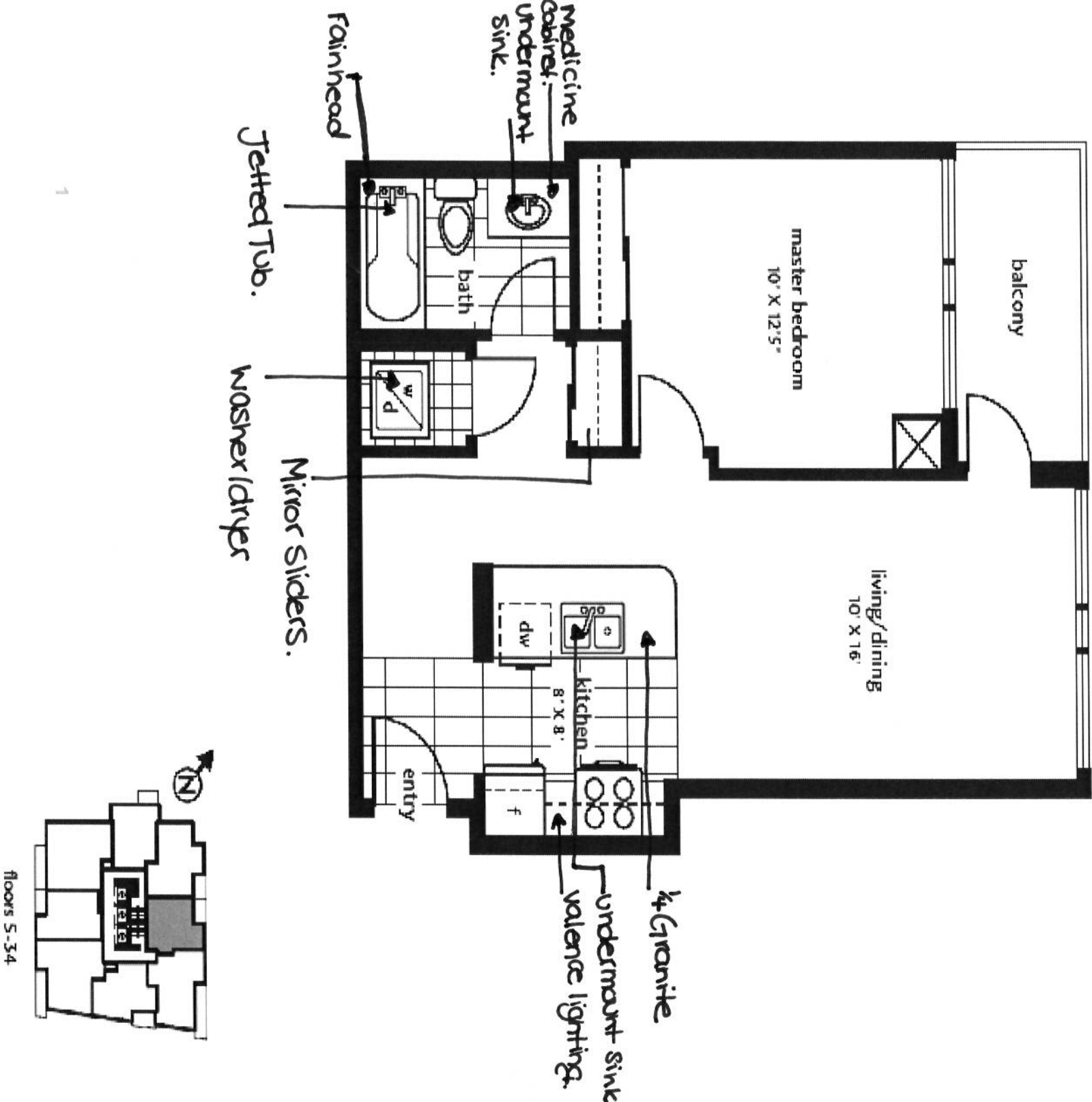
Floor Plan: LPH 1
