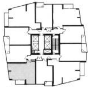
TYPICAL FLOOR
