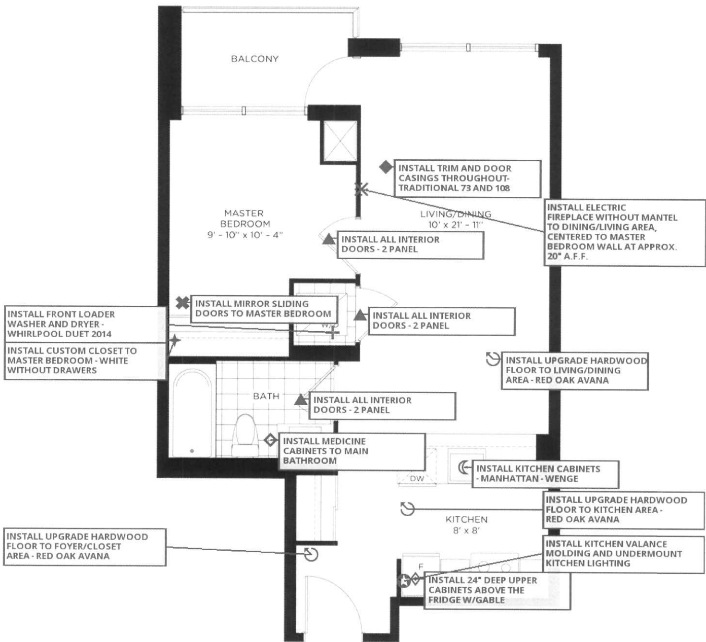
MAIN LEVEL
