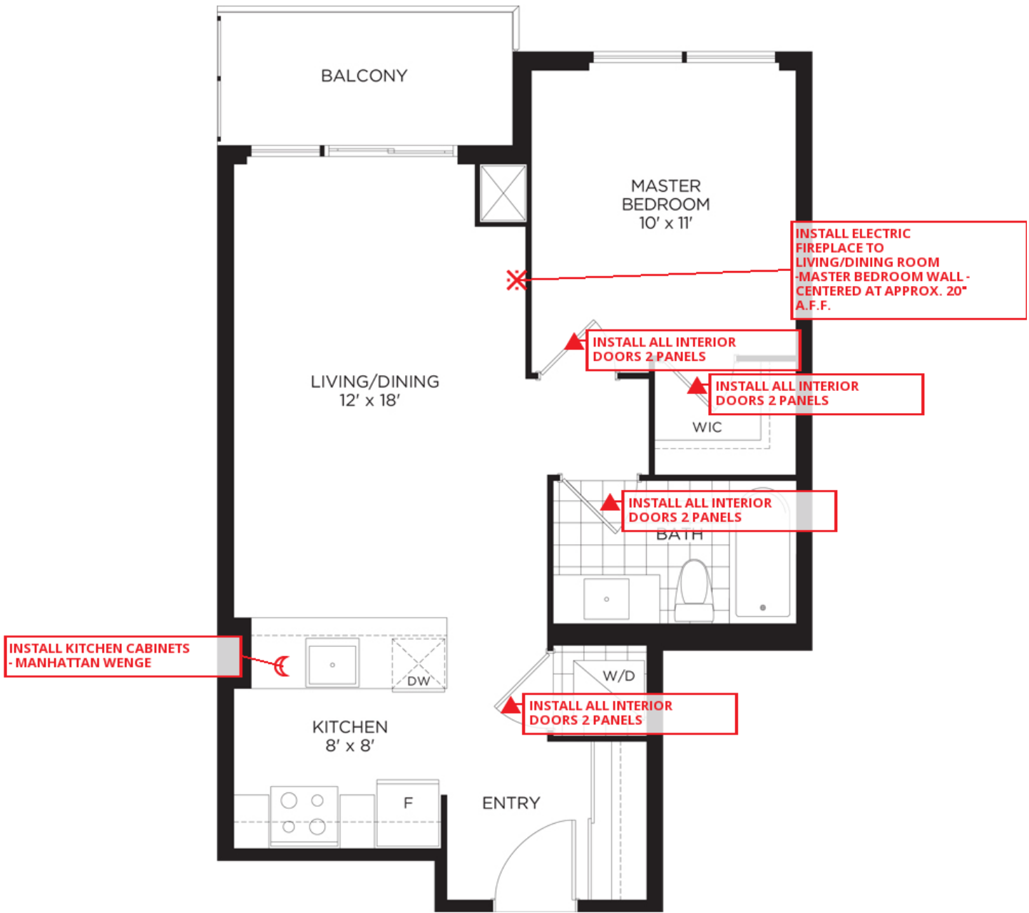
MAIN LEVEL
