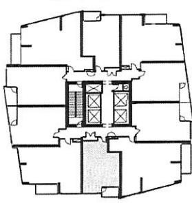
TYPICAL FLOOR
