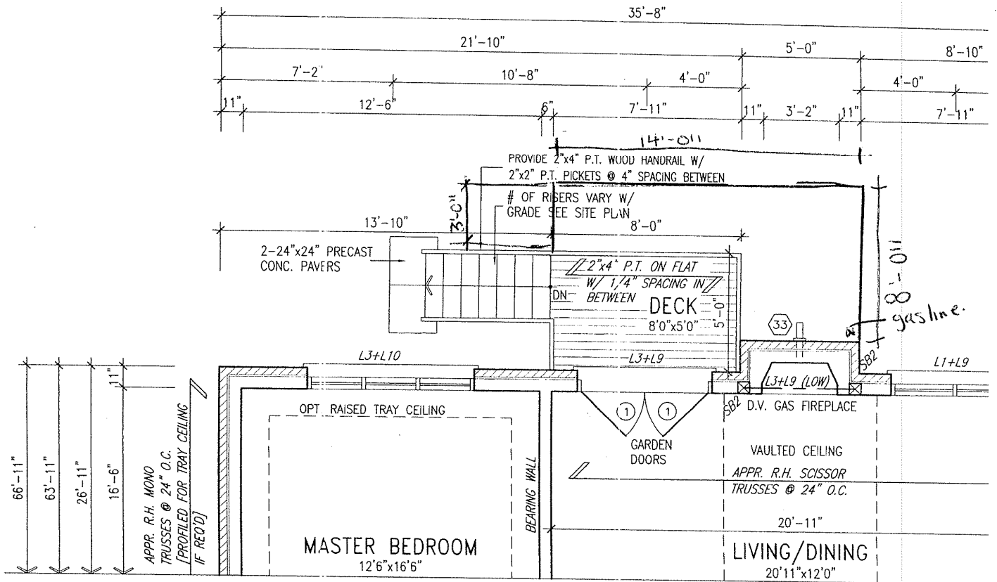
PART GRND FLOOR PLAN 'A' W.O.D. CONDITION ELEVS 'B' & 'C' SIMILAR
