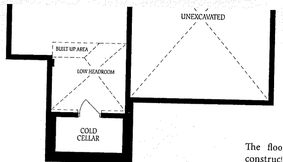
Basement Elevation B & C
