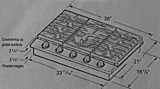
Cooktop Dimensions
