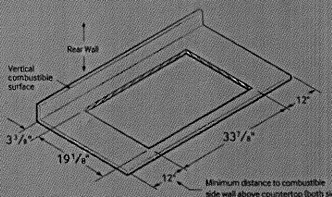
Cutout Dimensions of Countertop
