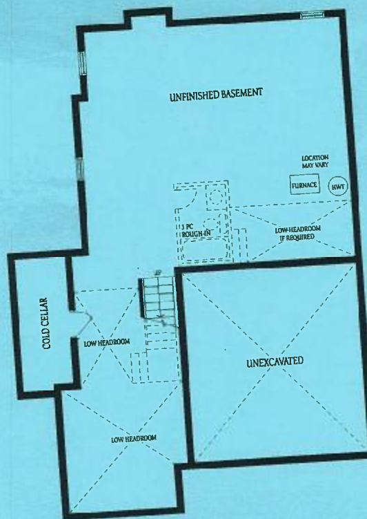
BASEMENT ELEVATION A
