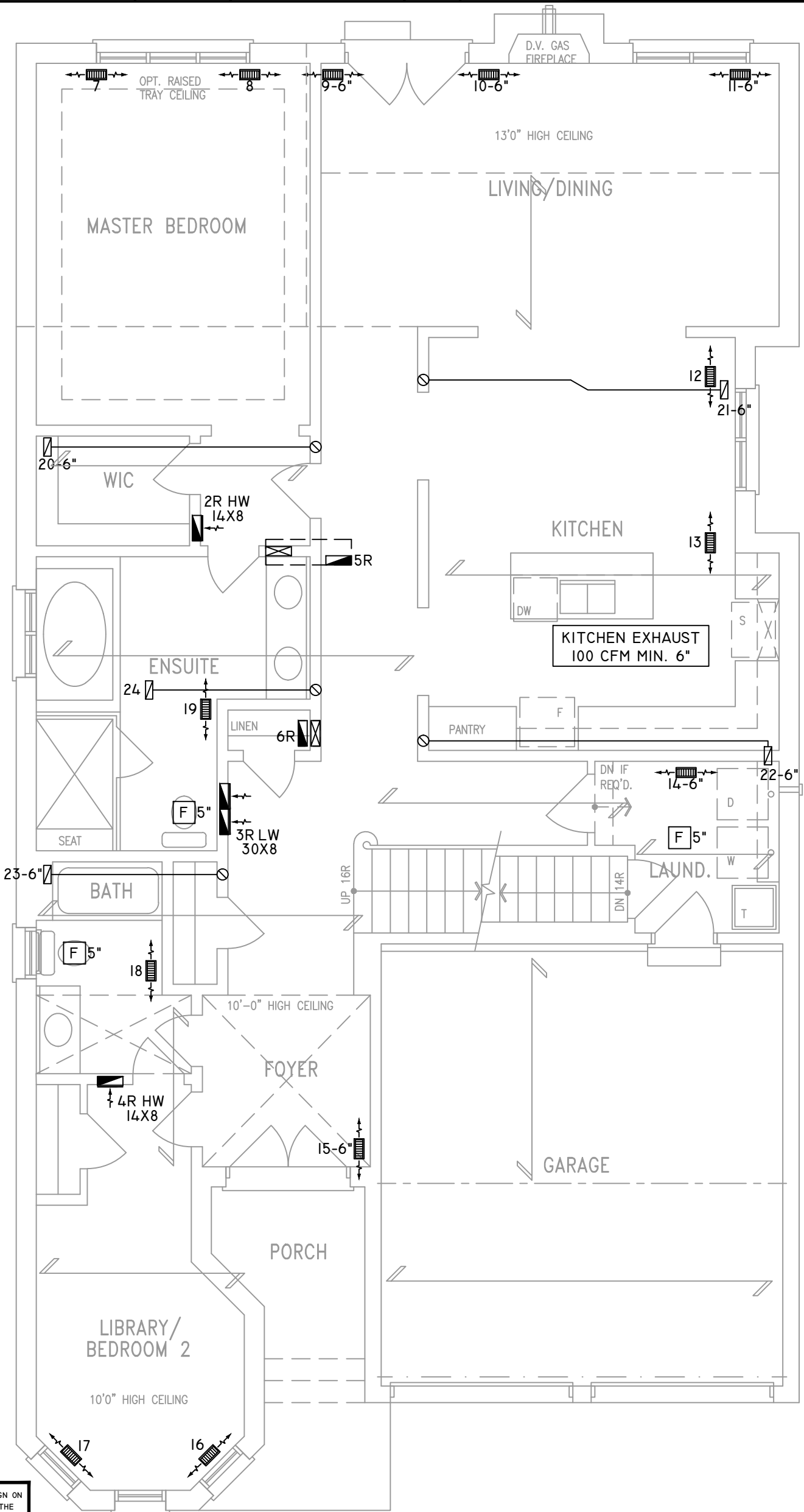
GROUND FLOOR PLAN 'A'
