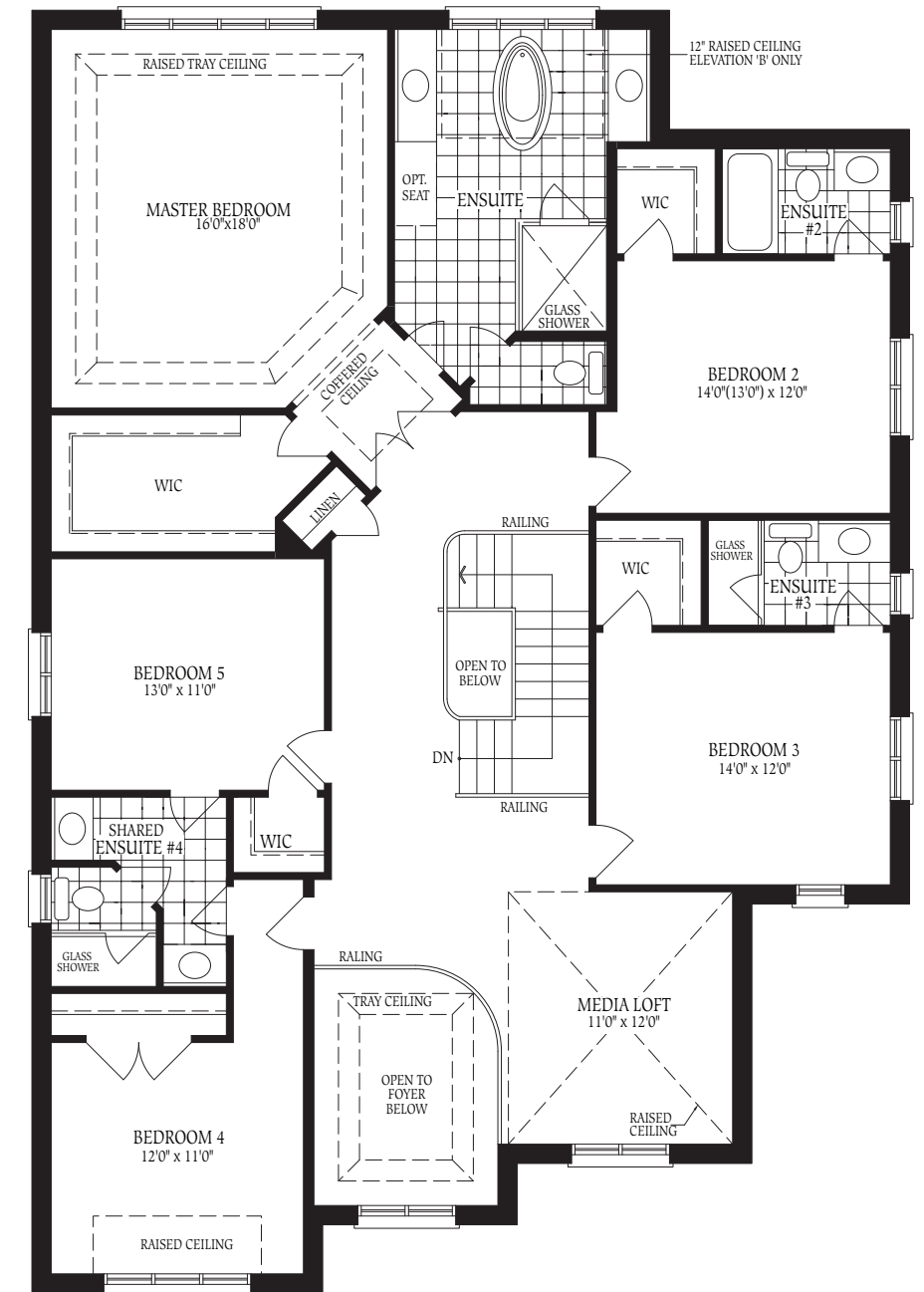
SECOND FLOOR PLAN 'A'
