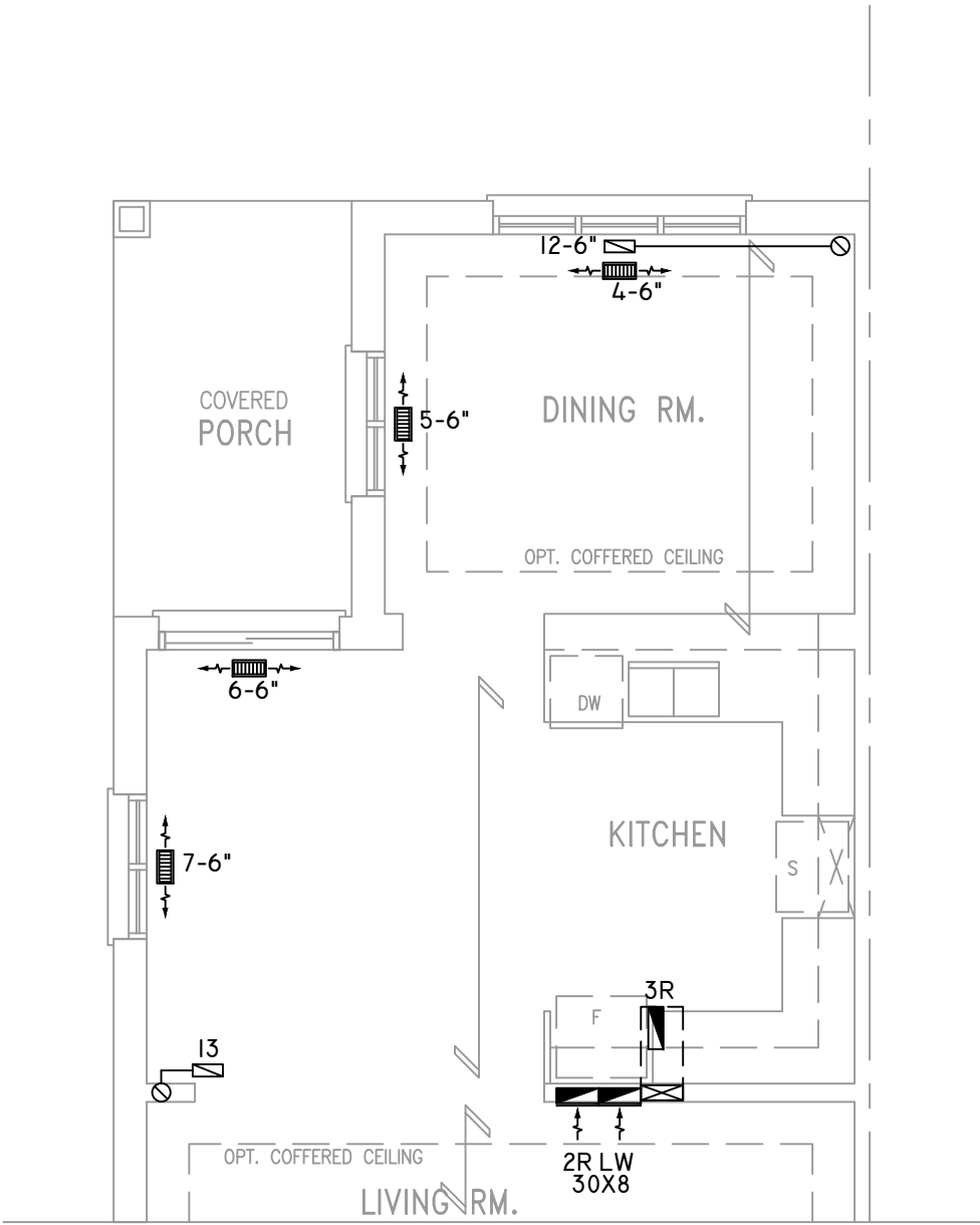
PART. OPT. ALT. GROUND FLOOR LAYOUT EL. 'A', 'B' & 'C'
