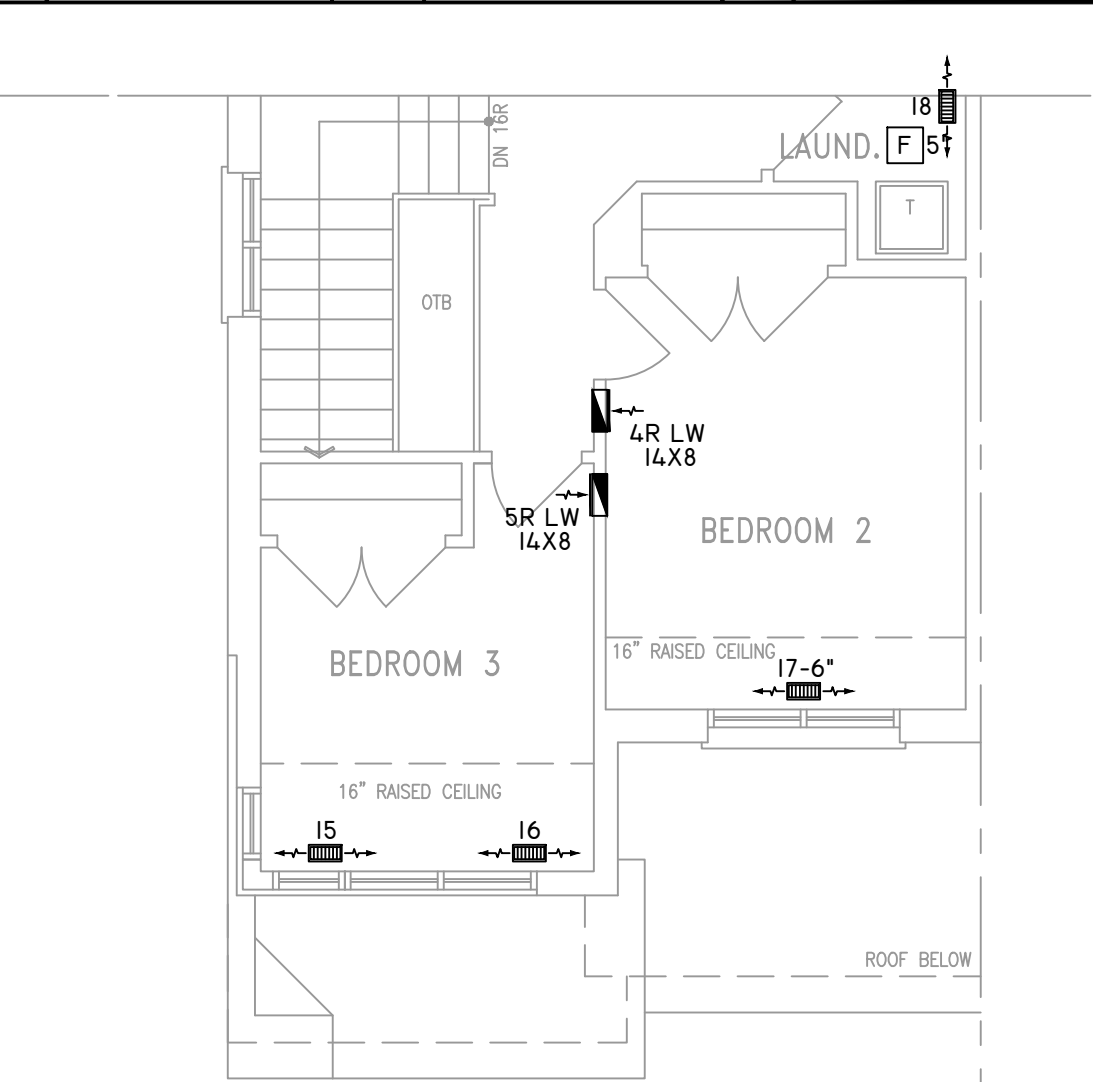
PART. SECOND FLOOR PLAN 'C MOD'
