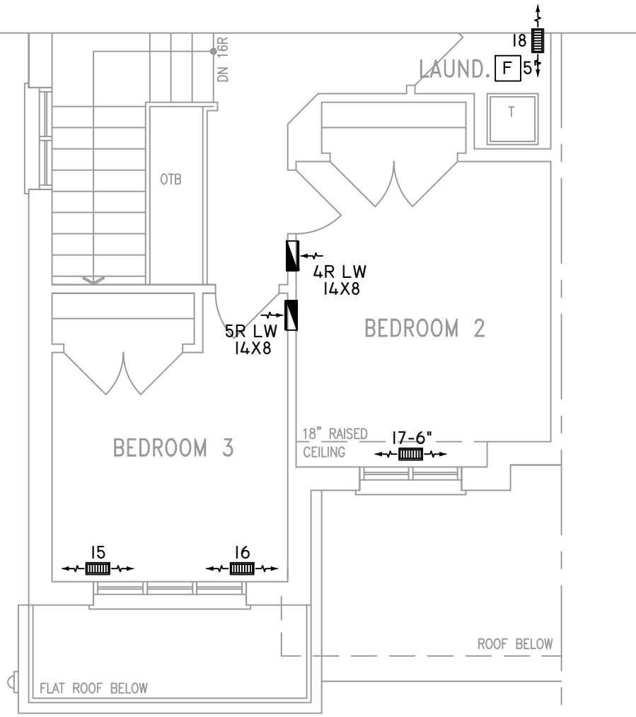
PART. SECOND FLOOR PLAN 'B'
