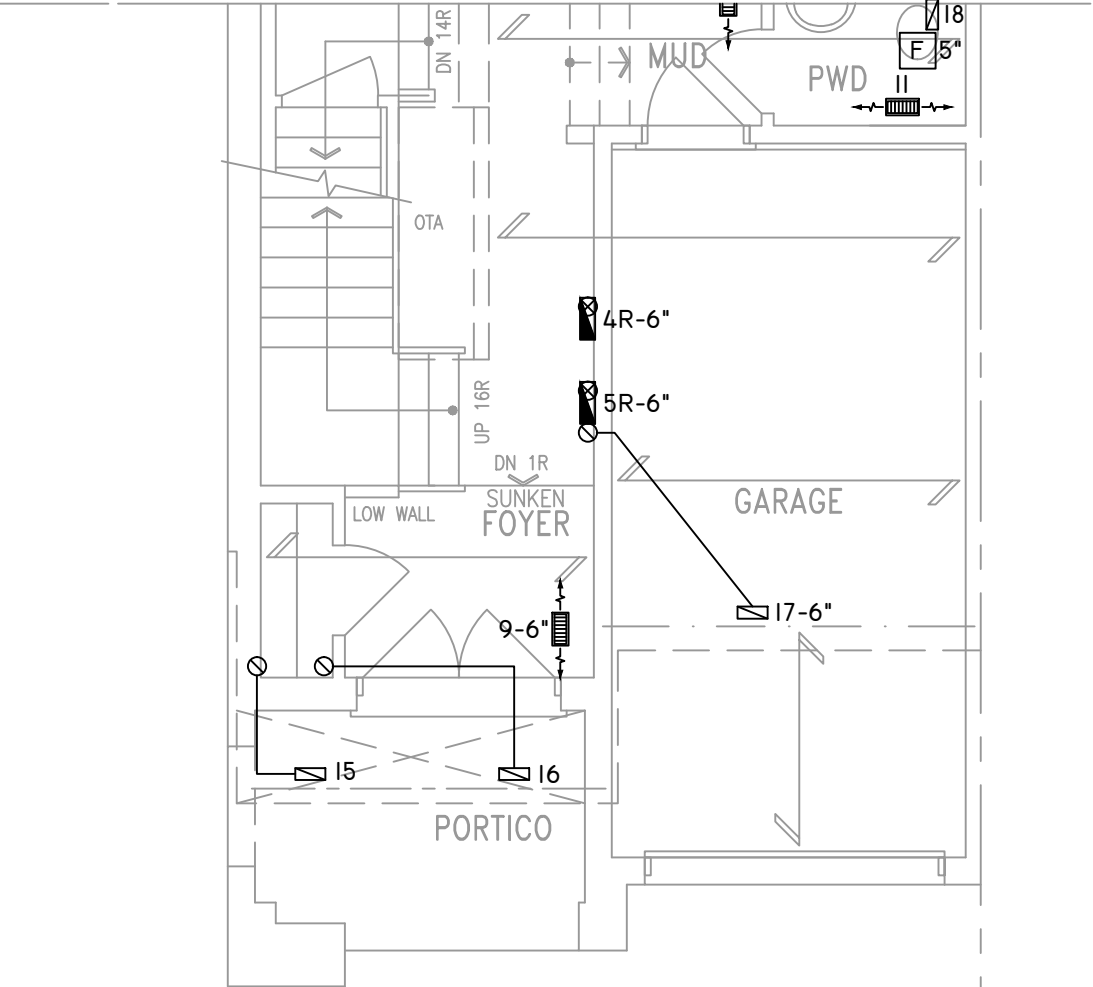
PART. GROUND FLOOR PLAN 'C MOD'
