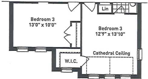
PARTIAL SECOND FLOOR PLAN ELEVATION C
