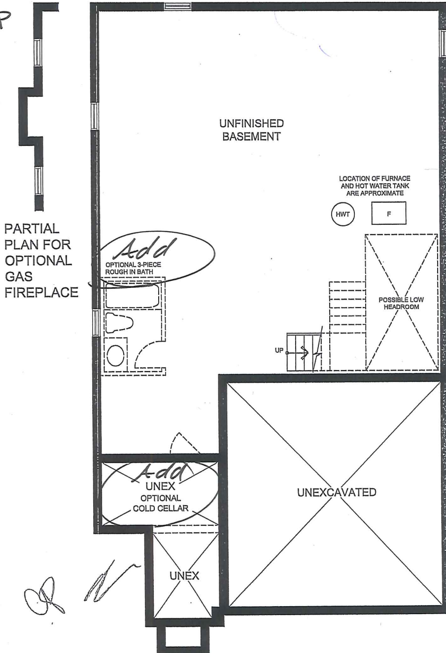
BASEMENT PLAN ELEVATION 'B'
