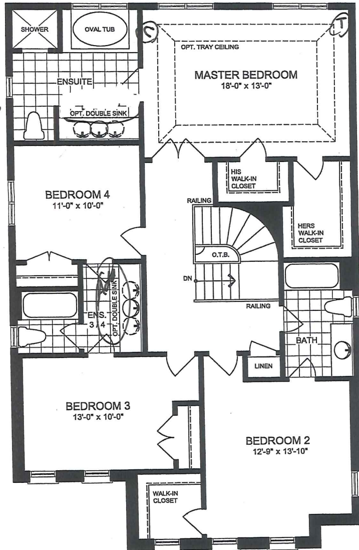
SECOND FLOOR PLAN ELEVATION 'A'
