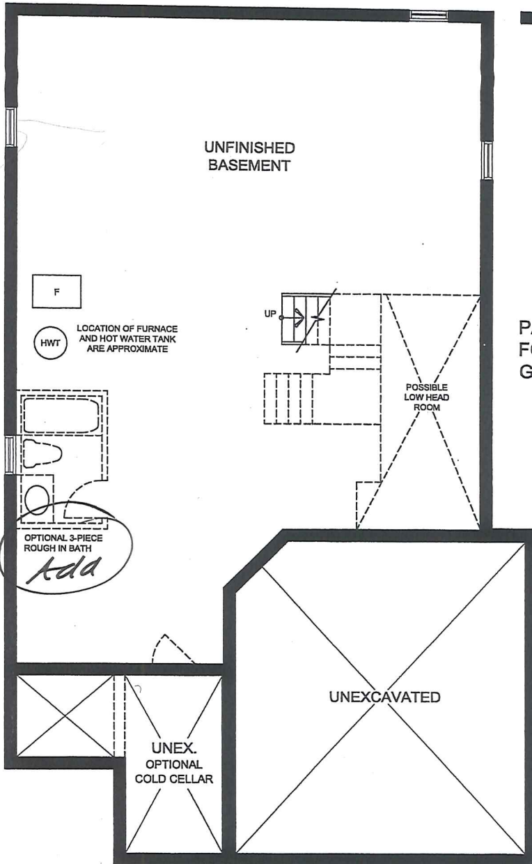
BASEMENT PLAN ELEVATION 'A'
