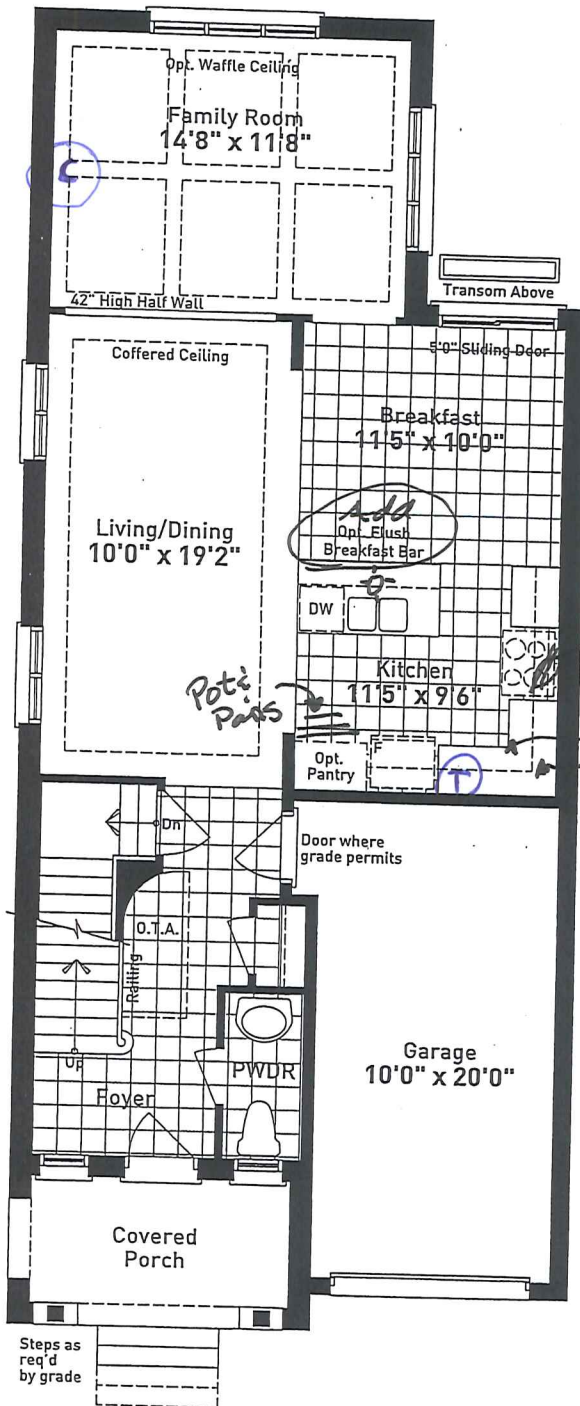
GROUND FLOOR PLAN ELEVATION A
