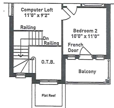
PARTIAL SECOND FLOOR PLAN ELEVATION C
