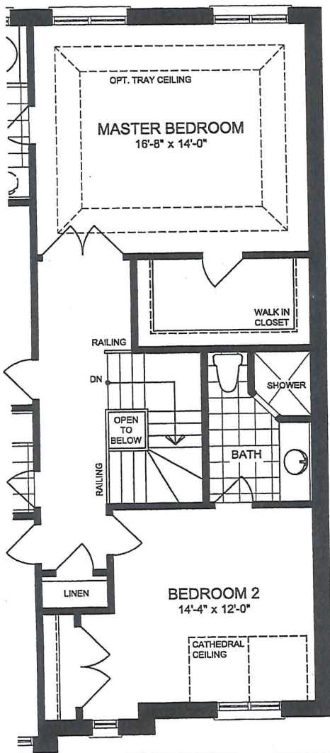
PARTIAL OPTIONAL SECOND FLOOR PLAN ELEVATION 'C' WITH BEDROOM 2 ENSUITE
