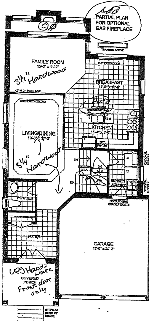
GROUND FLOOR PLAN ELEVATION 'B'
