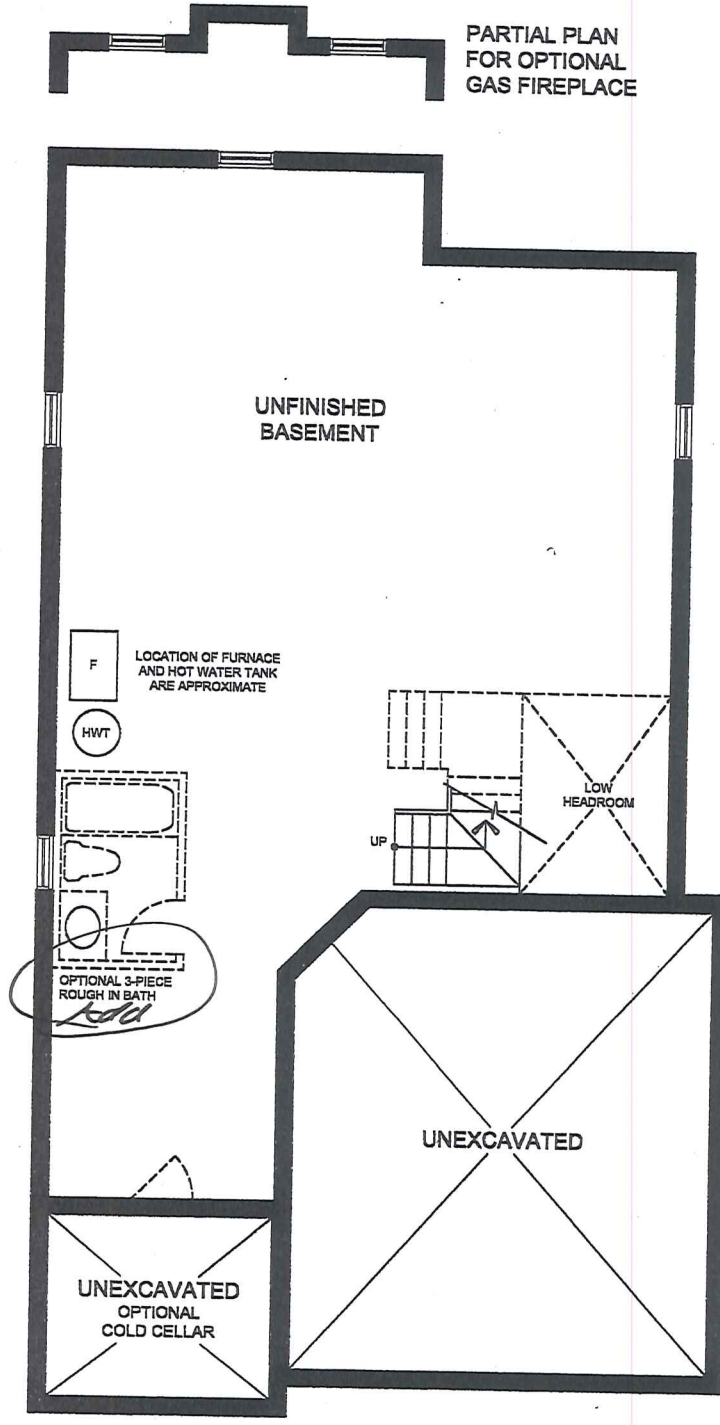
BASEMENT PLAN ELEVATION 'A' & 'B'
