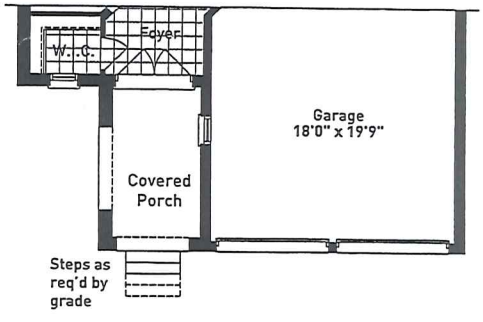
PARTIAL GROUND FLOOR PLAN ELEVATION B
