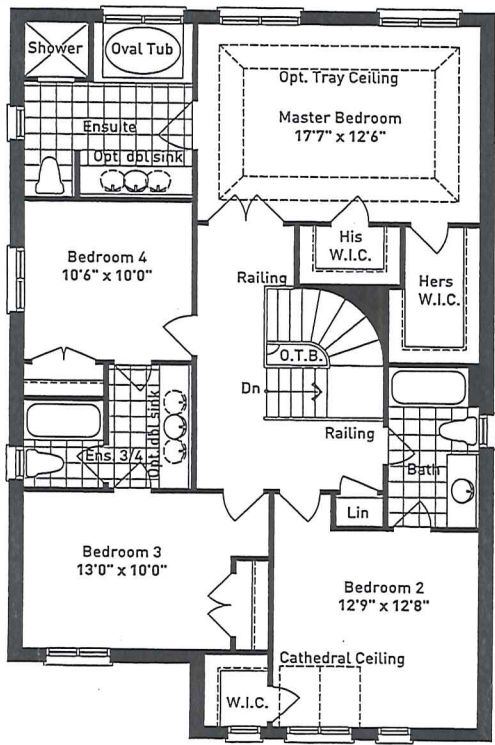
SECOND FLOOR PLAN ELEVATION B
