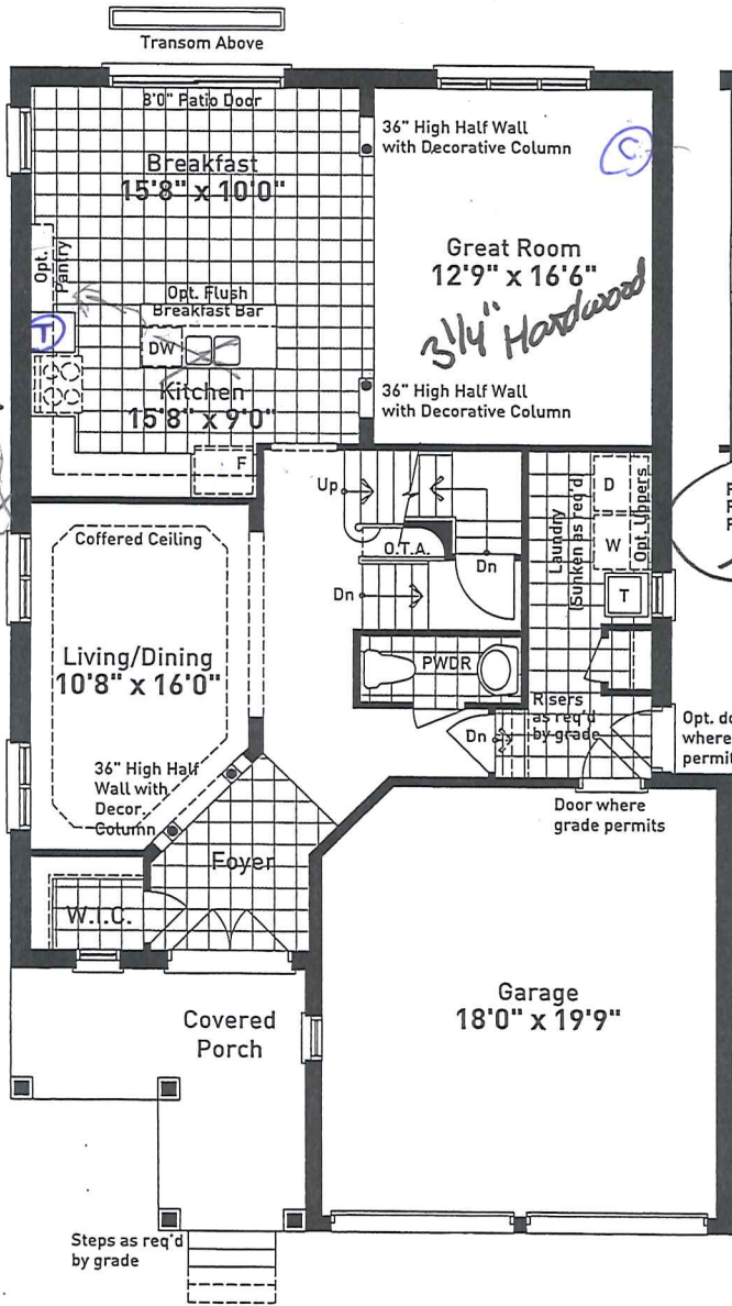
GROUND FLOOR PLAN ELEVATION A
