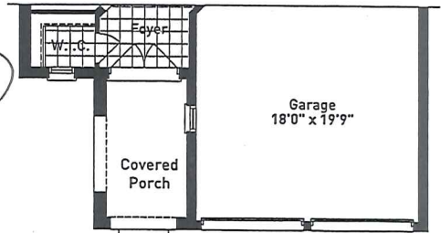
PARTIAL GROUND FLOOR PLAN ELEVATION B
