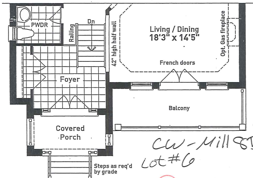
GROUND FLOOR PLAN ELEVATION C
