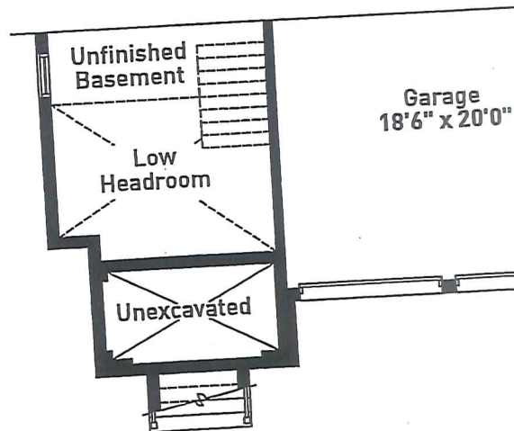
PARTIAL OPT. FINISHED BASEMENT FLOOR PLAN ELEVATION C
