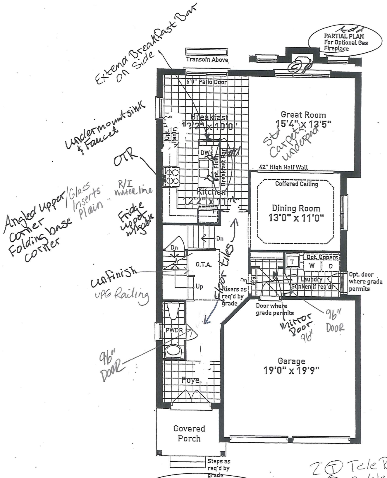
GROUND FLOOR PLAN ELEVATION A
