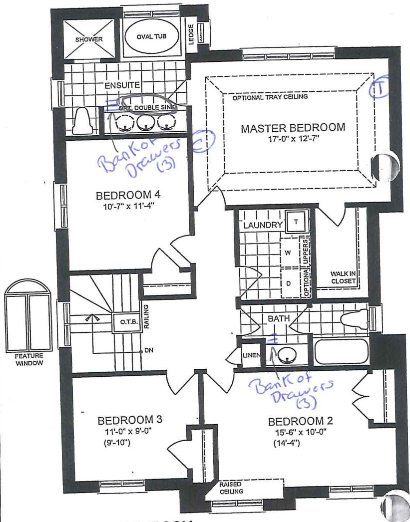
OPT. 4 BEDROOM SECOND FLOOR PLAN
