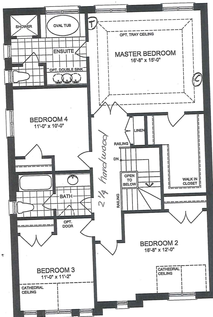
SECOND FLOOR PLAN ELEVATION 'C'
