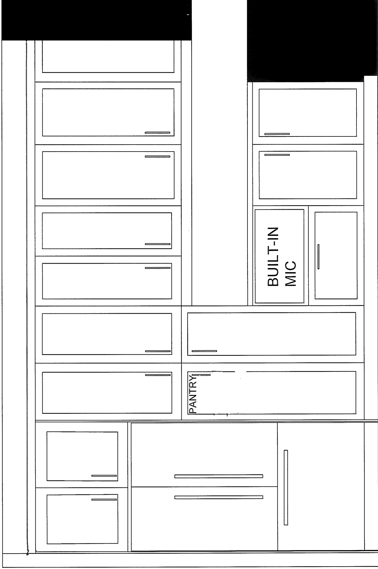
KITCHEN - ELEVATIONS
