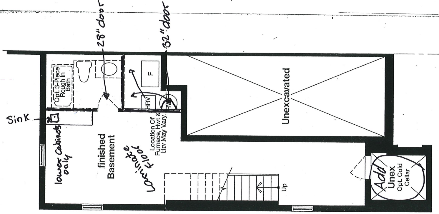
OPTION 3: OPTIONAL SECOND FLOOR LAUNDRY LAYOUT
