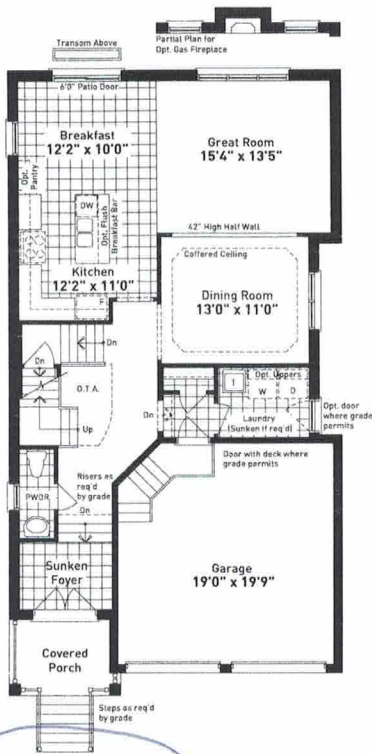
GROUND FLOOR PLAN ELEVATION B
