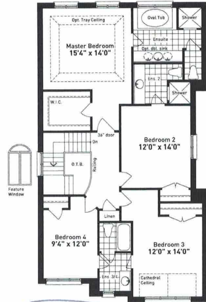
SECOND FLOOR PLAN ELEVATION B
