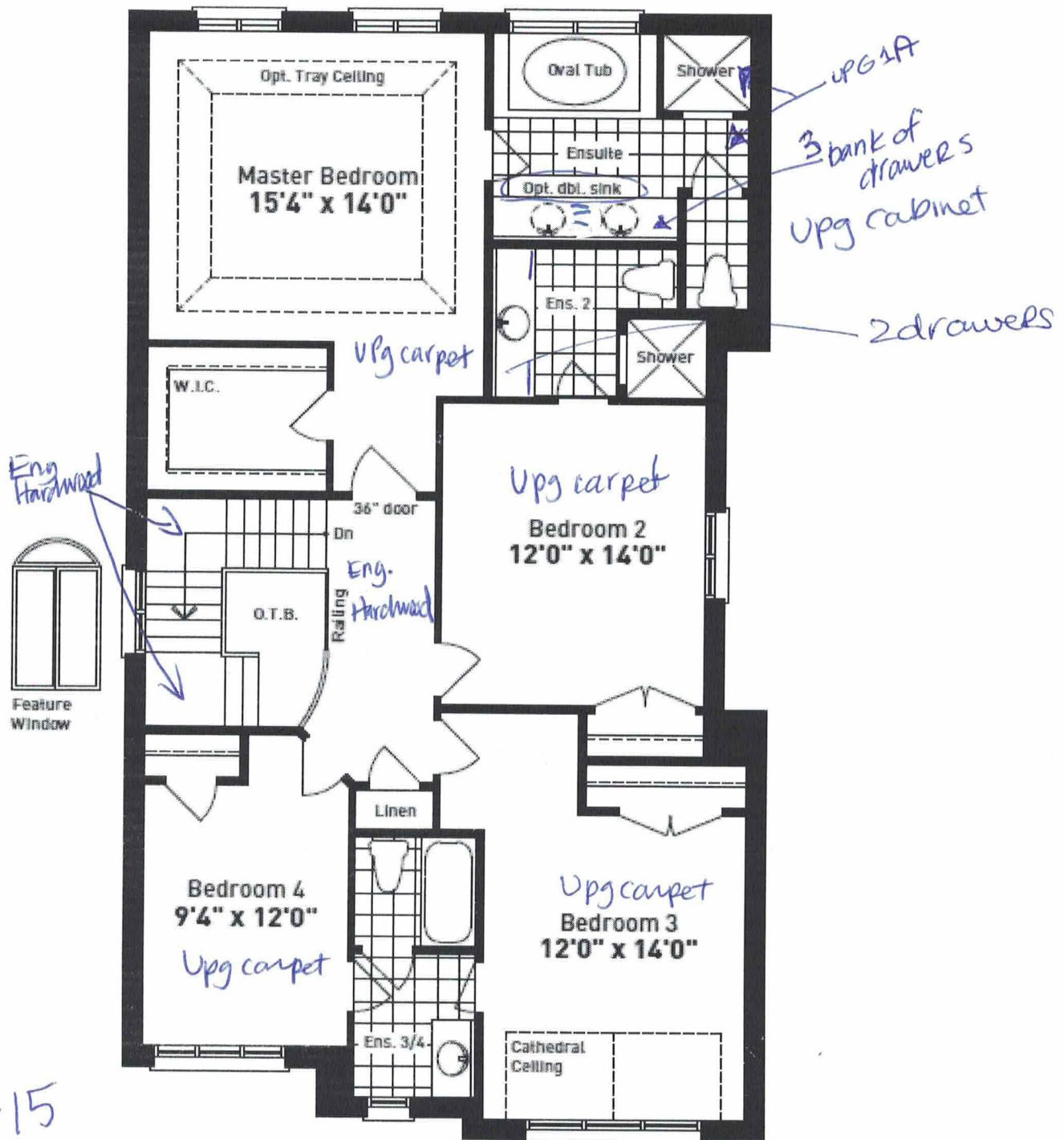
SECOND FLOOR PLAN ELEVATION B
