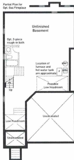
PARTIAL BASEMENT FLOOR PLAN ELEVATION C
