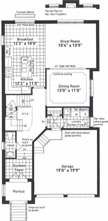
GROUND FLOOR PLAN ELEVATION C
