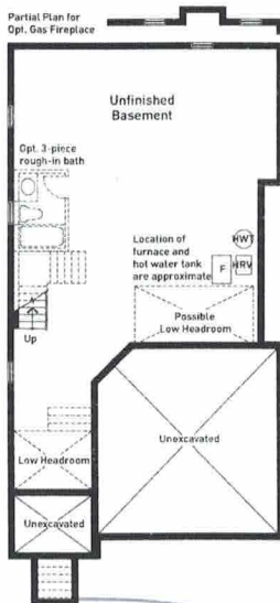
BASEMENT FLOOR PLAN ELEVATION B
