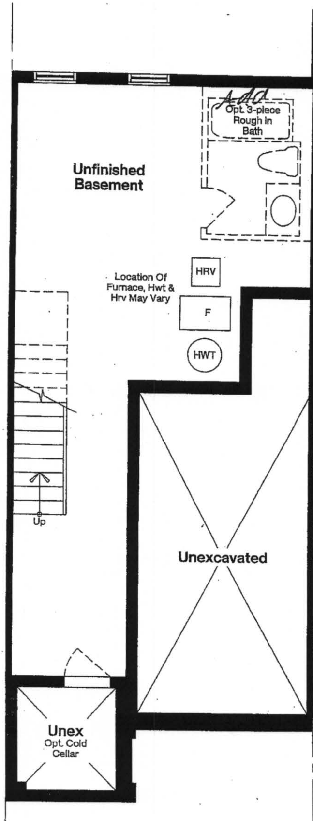
BASEMENT PLAN
