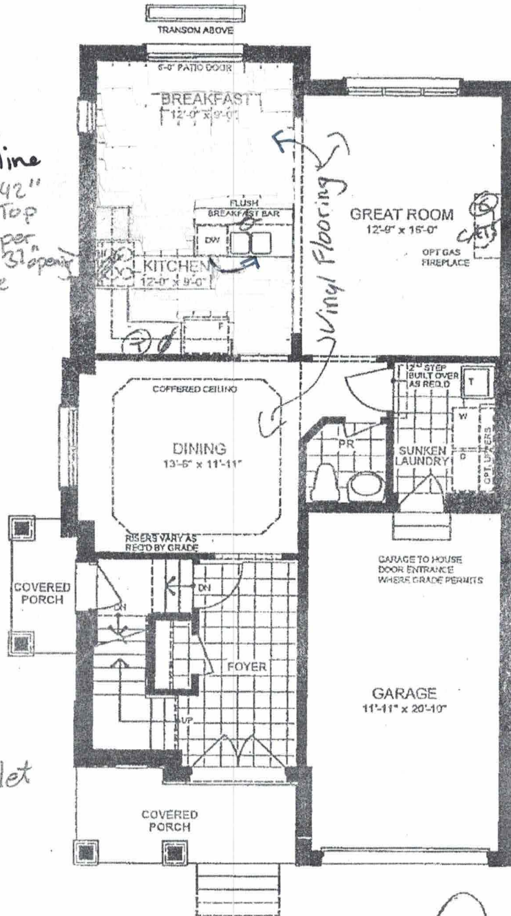
GROUND FLOOR PLAN ELEVATION B
