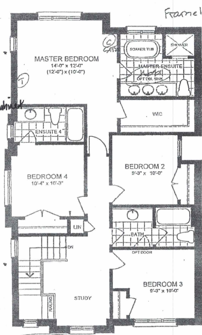
SECOND FLOOR PLAN ELEVATION B
