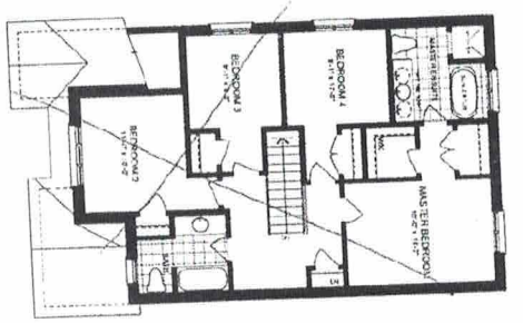
SECOND FLOOR PLAN ELEVATION A
