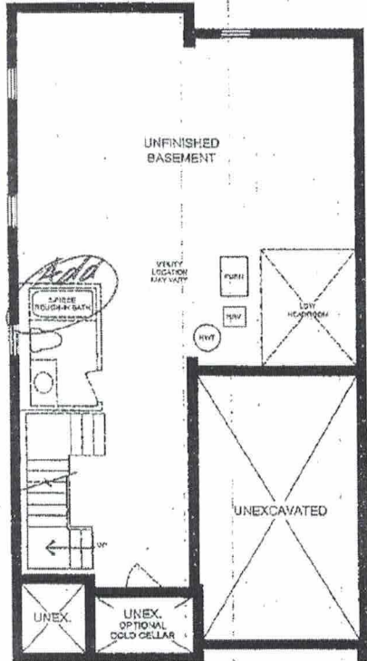
BASEMENT PLAN ELEVATION A
