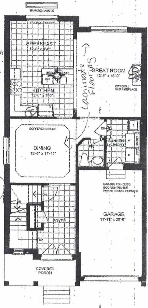
GROUND FLOOR PLAN ELEVATION A
