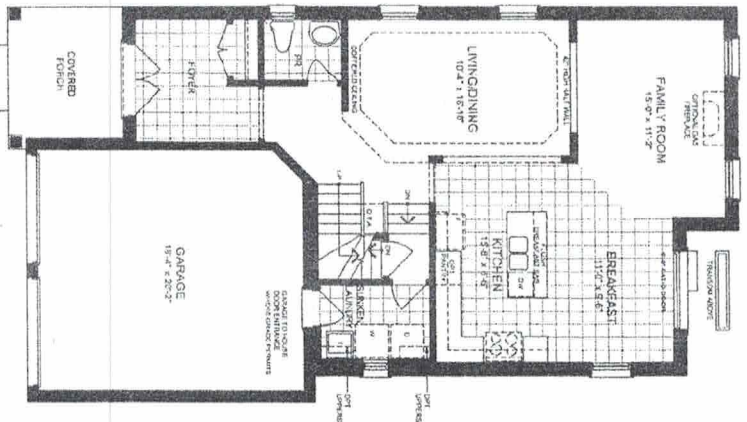
GROUND FLOOR PLAN ELEVATION A
