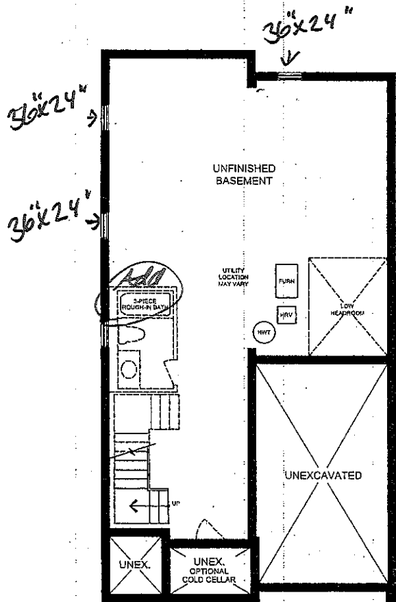
BASEMENT PLAN ELEVATION A
