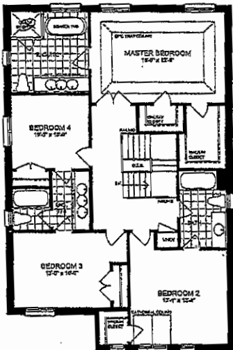
SECOND FLOOR PLAN ELEVATION A
