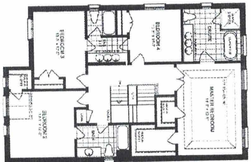
SECOND FLOOR PLAN ELEVATION A
