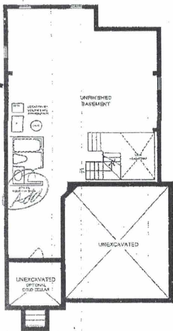
BASEMENT PLAN ELEVATION A
