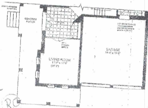
PARTIAL GROUND FLOOR PLAN ELEVATION B
