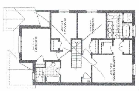
SECOND FLOOR PLAN ELEVATION A
