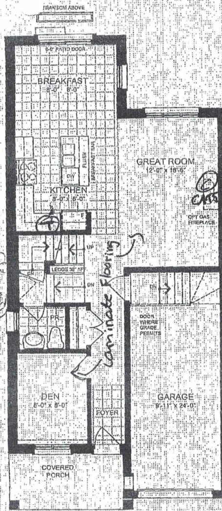
GROUND FLOOR PLAN ELEVATION A1, A2, & B
