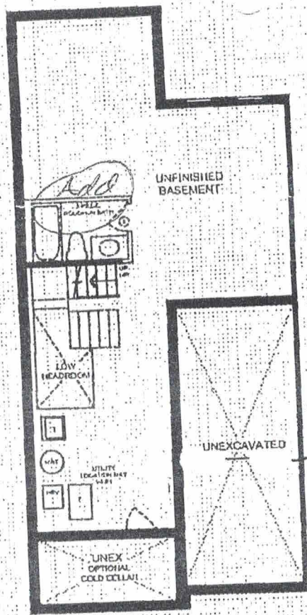
BASEMENT PLAN ELEVATION A1, A2 & B
