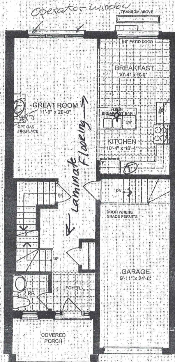
GROUND FLOOR PLAN ELEVATION A & B
