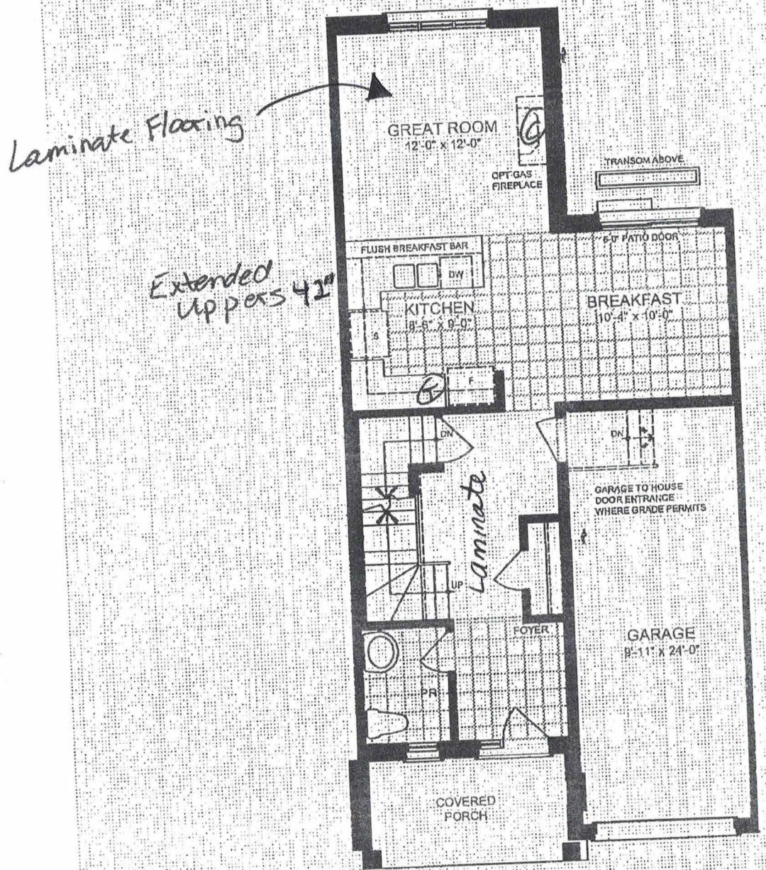
GROUND FLOOR PLAN ELEVATION A & B
