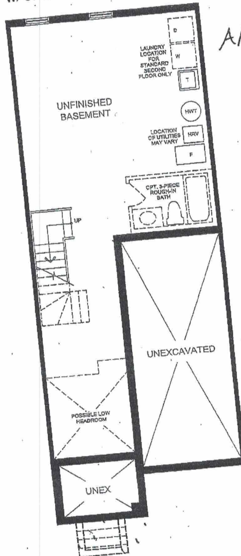
BASEMENT PLAN ELEVATION A
