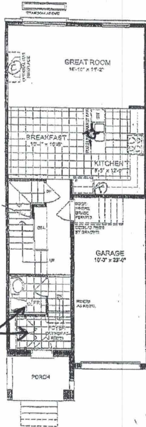
GROUND FLOOR PLAN ELEVATION A
