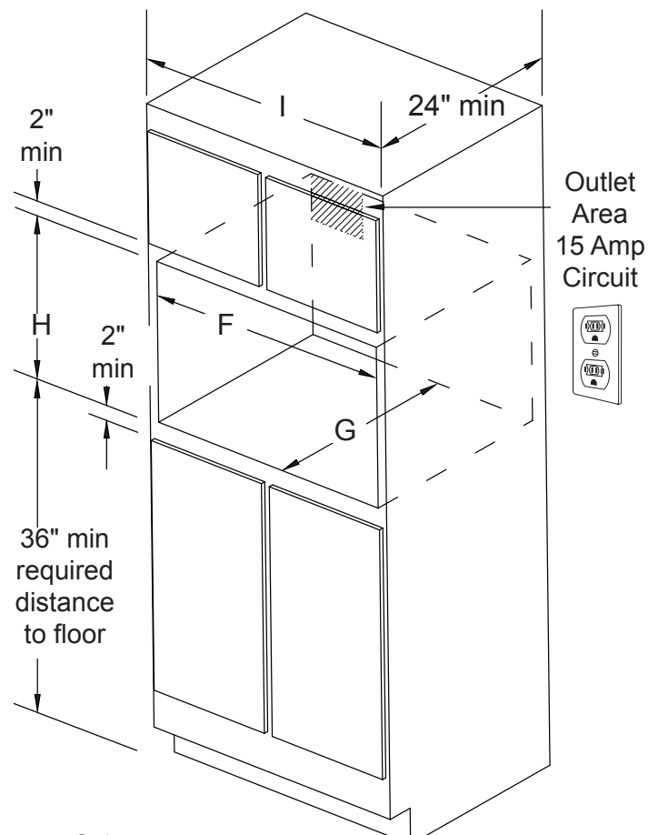
Figure 2: Microwave Only
