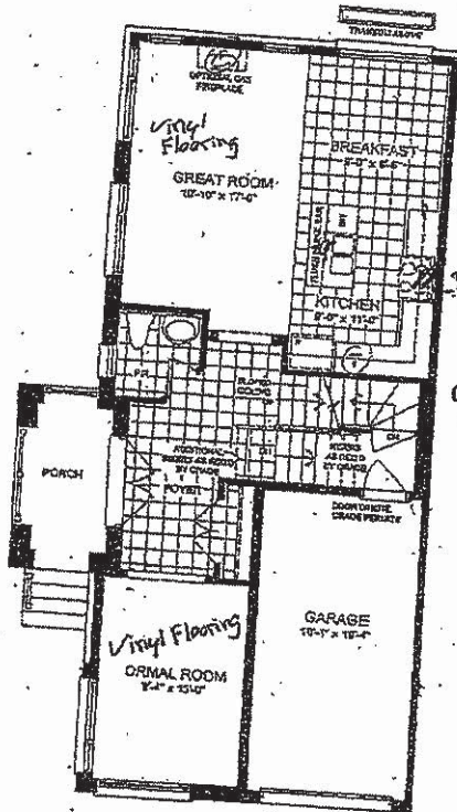
GROUND FLOOR PLAN ELEVATION A
