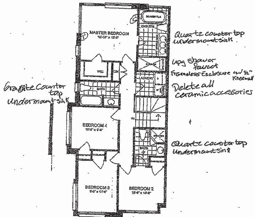
OPTIONAL SECOND FLOOR PLAN ELEVATION A
