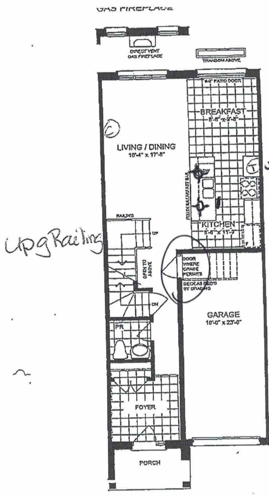
GROUND FLOOR PLAN ELEVATION RI
