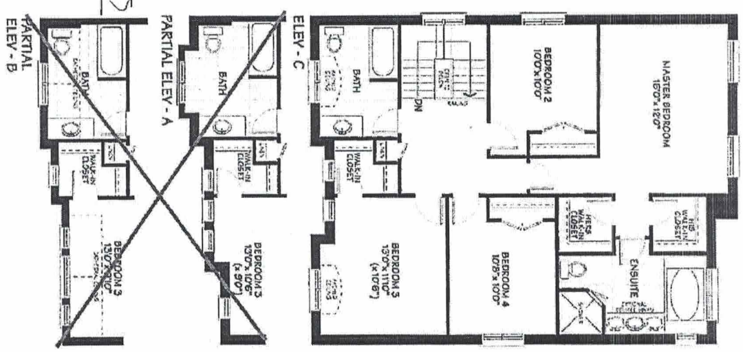
SECOND FLOOR
